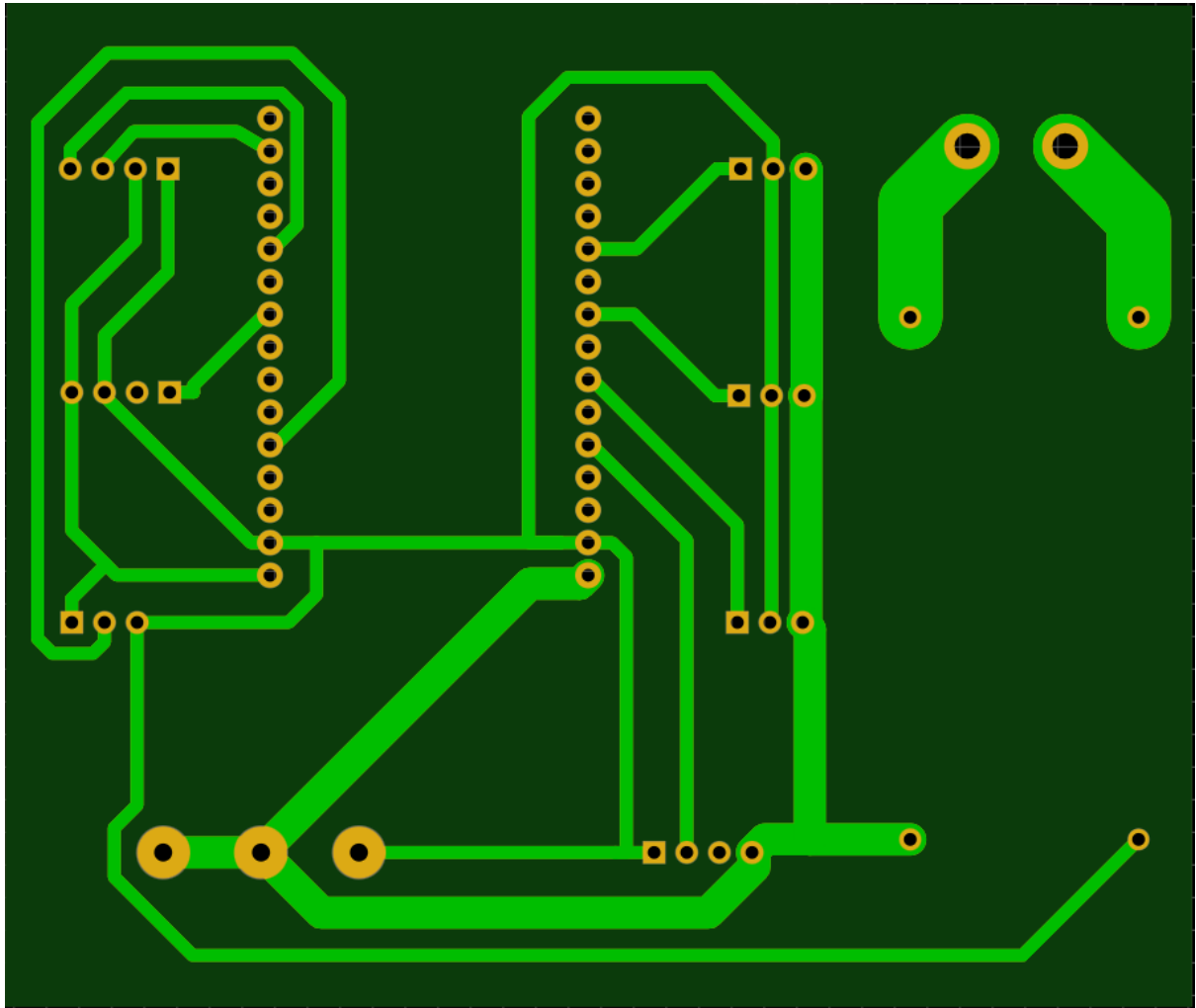
PCB Bottom Layer:
