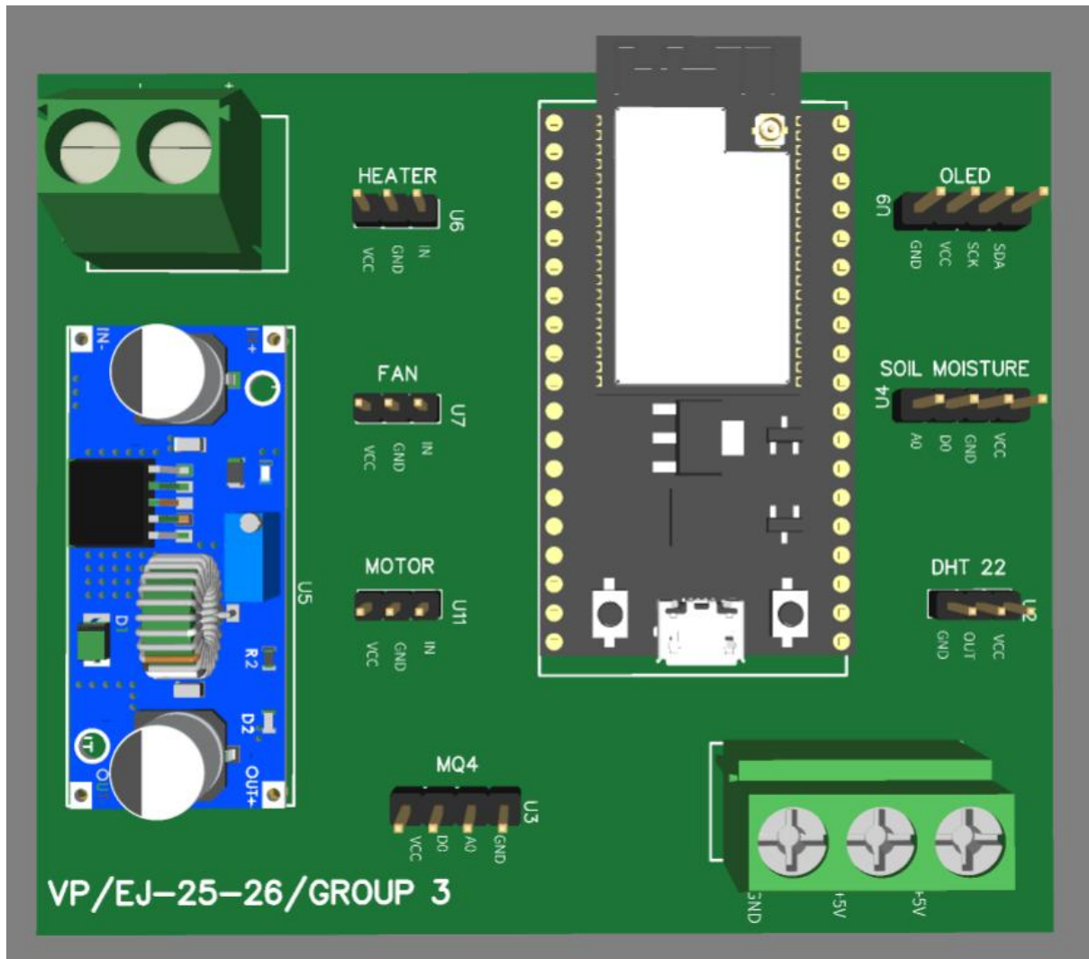
PCB 3D View:
